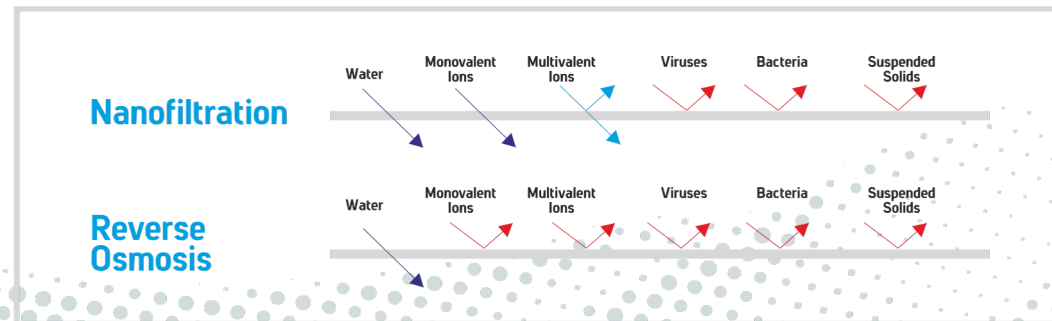
Use Nano Filtration Membrane for Drinking Water
